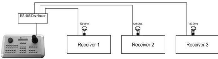
Star wiring with RS-485 signal distributor
