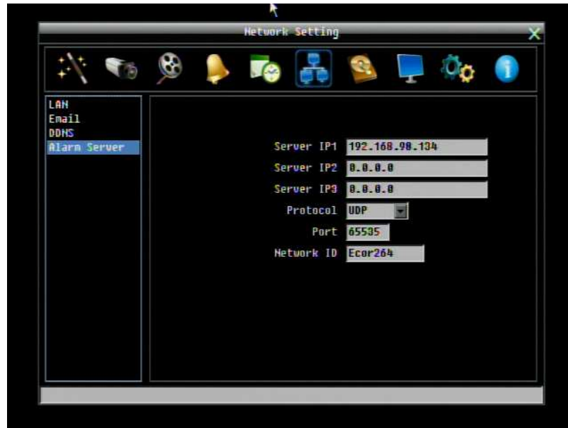
Figure 4-29 Network Menu – Alarm Server
