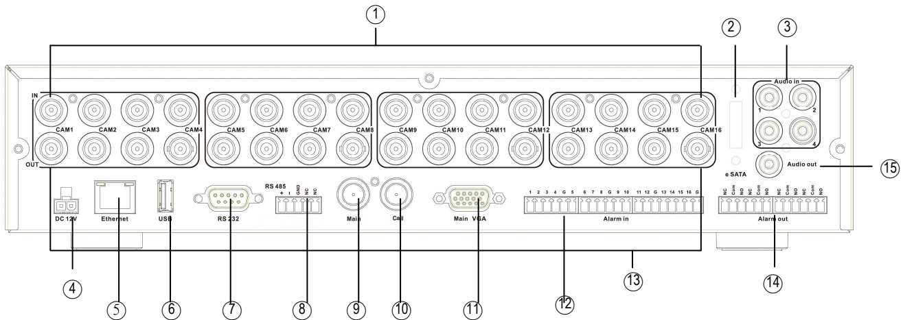
Figure 1-2 Rear Panel
