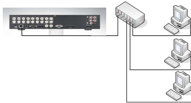
Figure 1-4 Network Connection through Patch Cable
